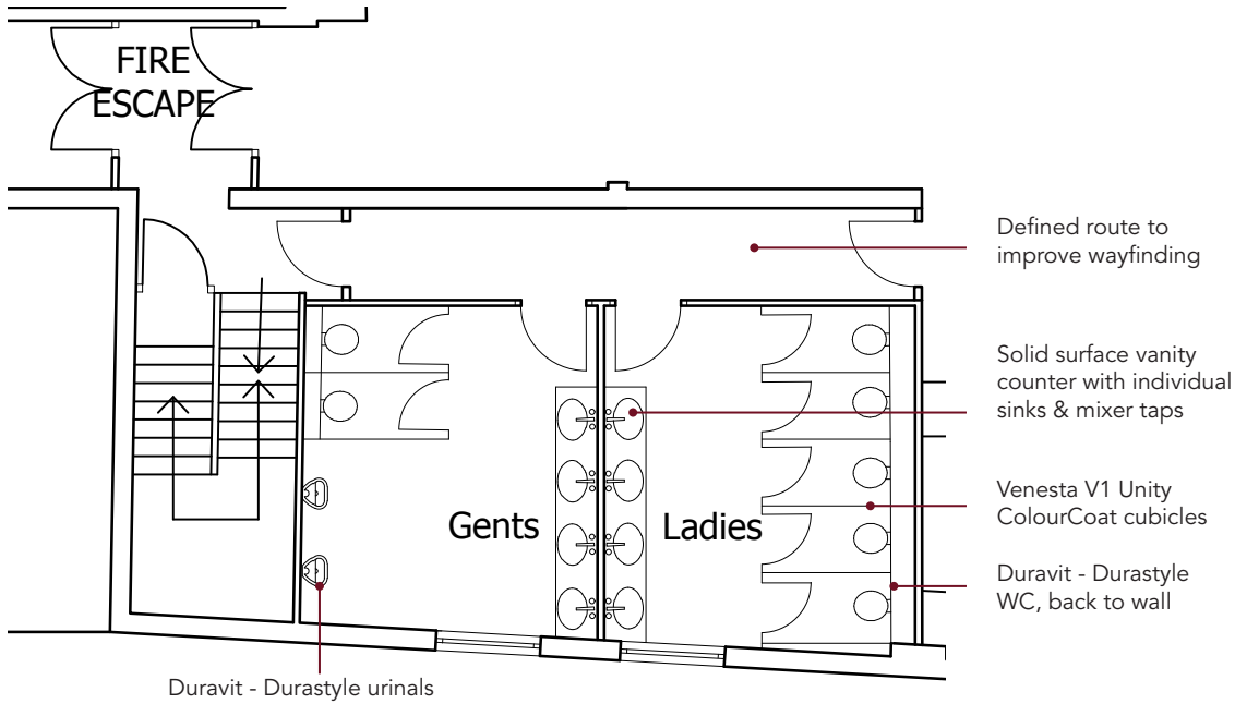
Proposed plan - 2 gents toilets, 2 urinals and 5 ladies toilets
